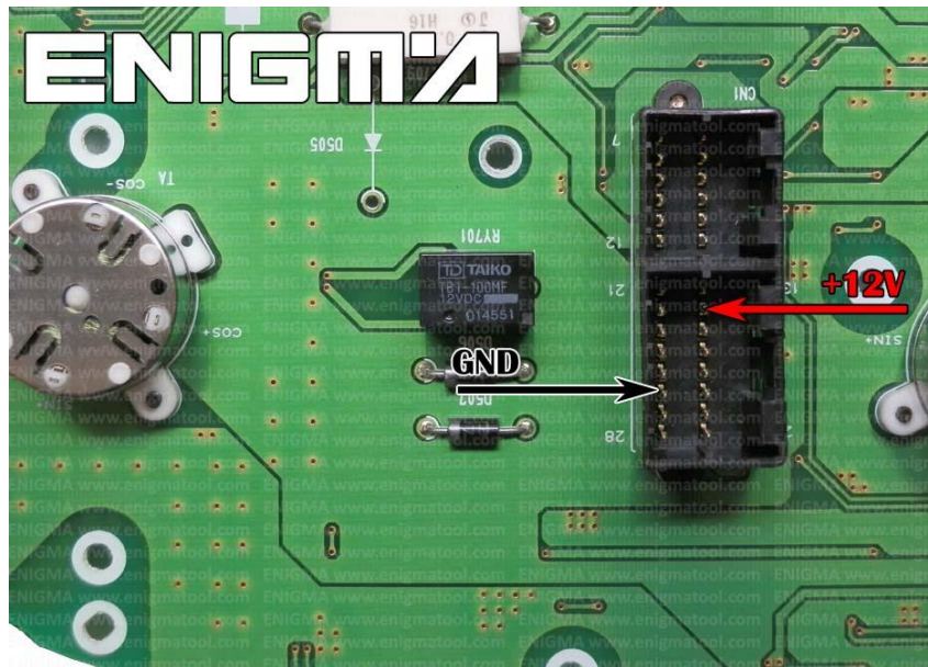
PHOTO 2: Power connection.
