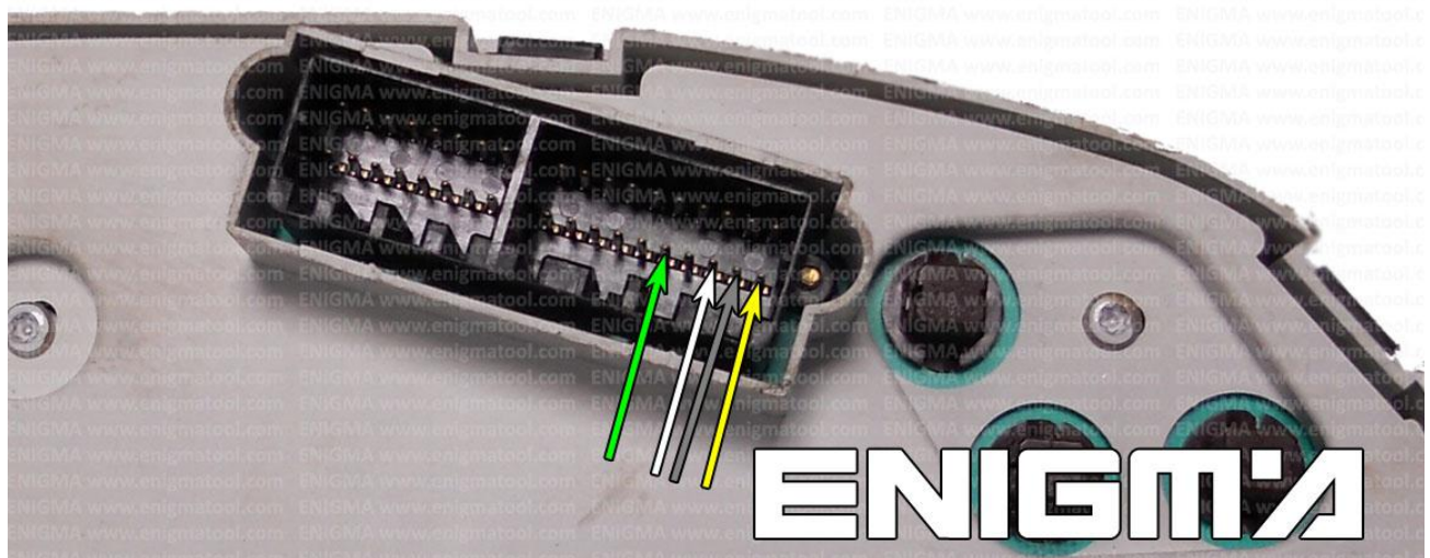
PHOTO 1: Solder cables according to the colors like shown on the photo above.
