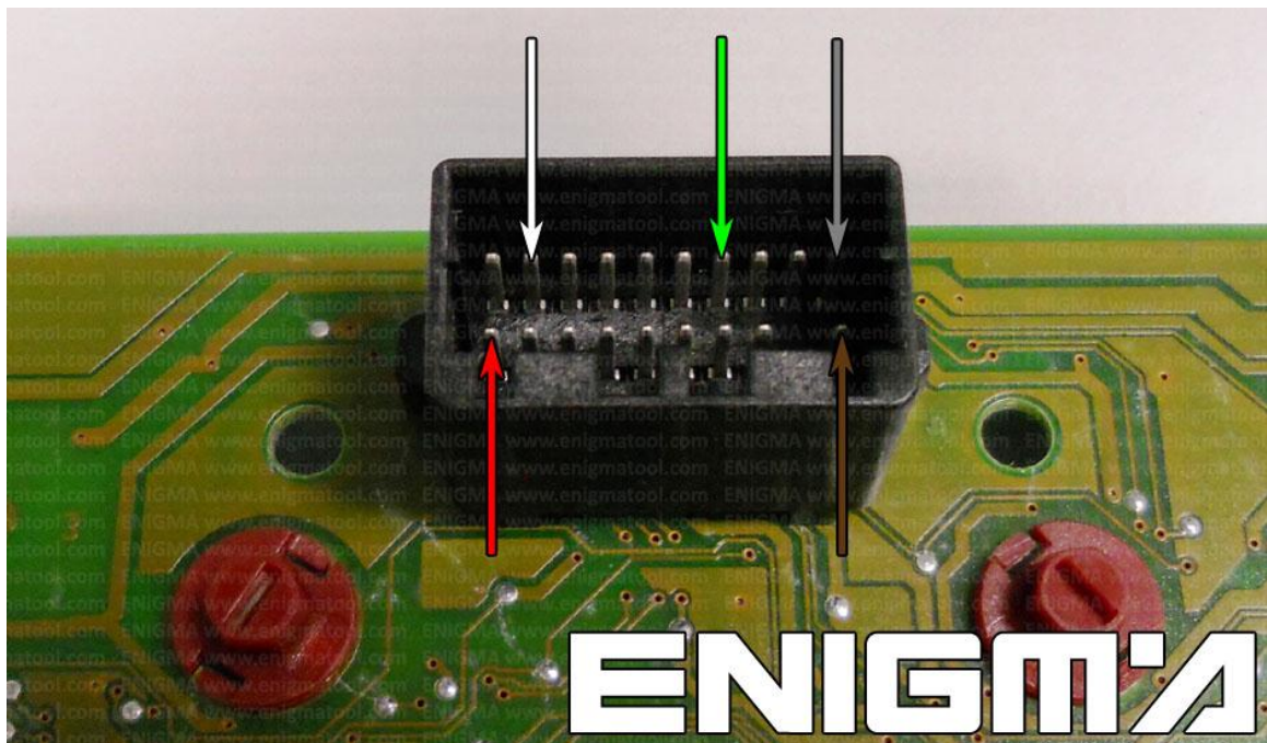
PHOTO 1: Connect C29 cables according to the picture above.
