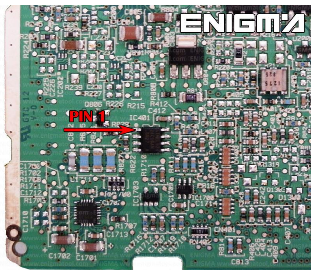
PHOTO 1: Connect cable C4 to the EEPROM memory according to the picture above.
