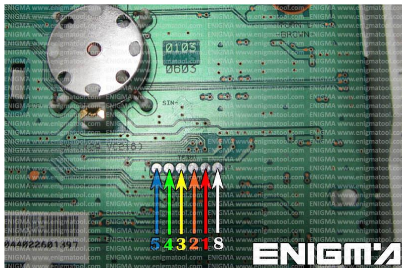
PHOTO 1: Solder cables according to the colors like shown on the photo above.
