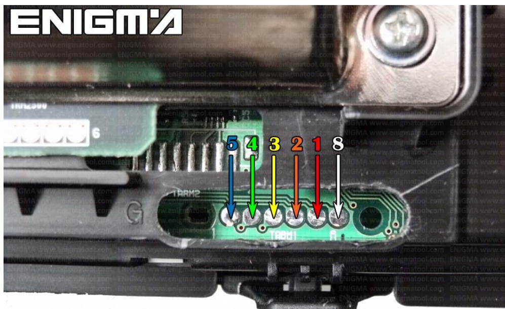
PHOTO 1: Connect cable C7 to the points as shown on the picture above.
