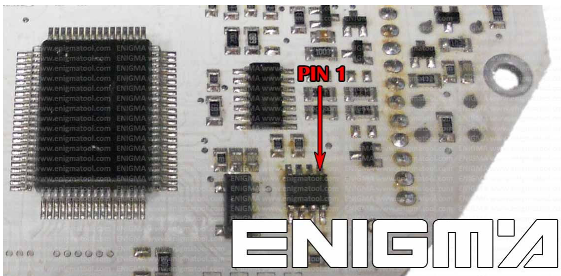
PHOTO 1: Connect cable C4 to the Eeprom memory according to the picture above.
