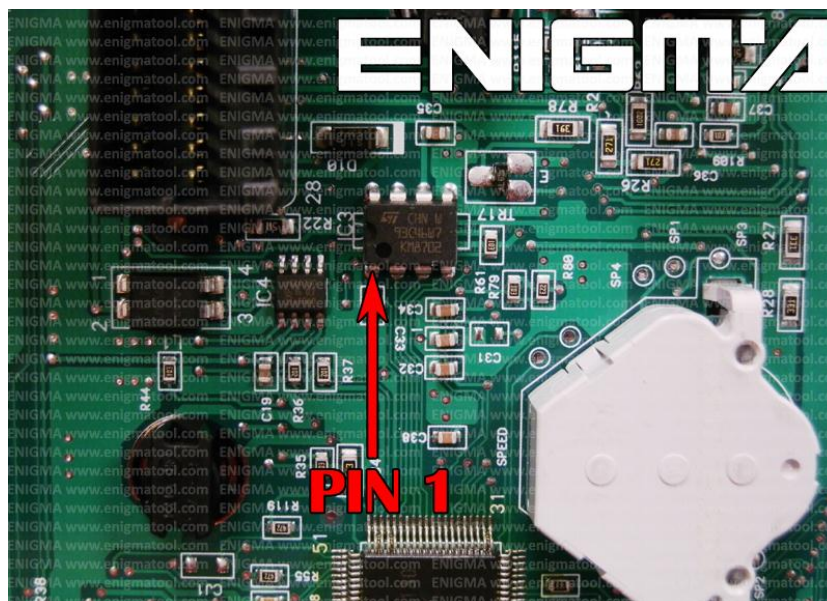
PHOTO 1: Connect cable C5 to the EEPROM memory according to the picture above.
