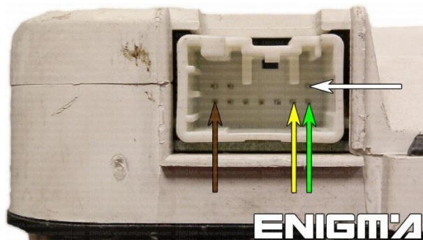
PHOTO 1: Connect cable C41 according to the colors like shown on the photo above.
