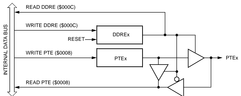
Figure 20-15. Port E I/O Circuit
