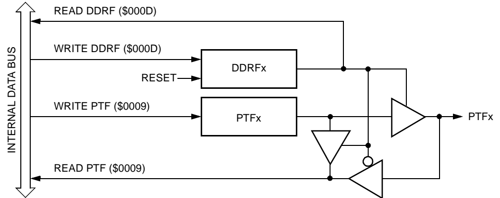
Figure 20-18. Port F I/O Circuit
