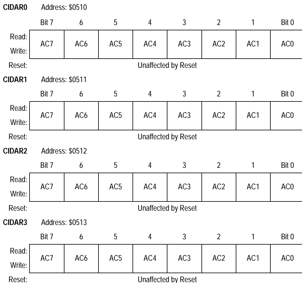
Figure 21-26. Identifier Acceptance Registers (CIDAR0–CIDAR3)
