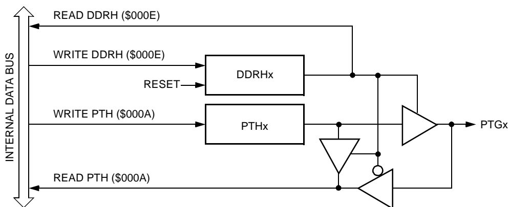
Figure 20-24. Port H I/O Circuit
