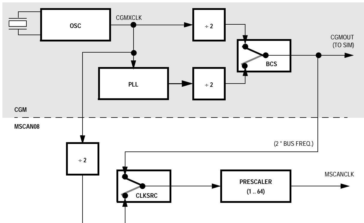
Figure 21-7. Clocking Scheme
