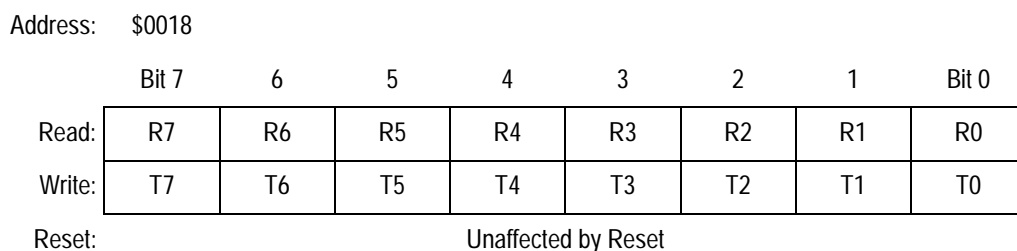
Figure 16-17. SCI Data Register (SCDR)
