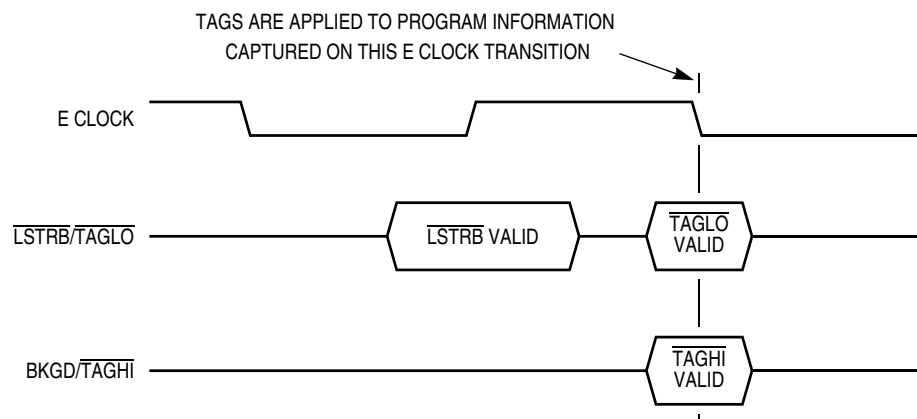
Figure 8-5. Tag Input Timing
