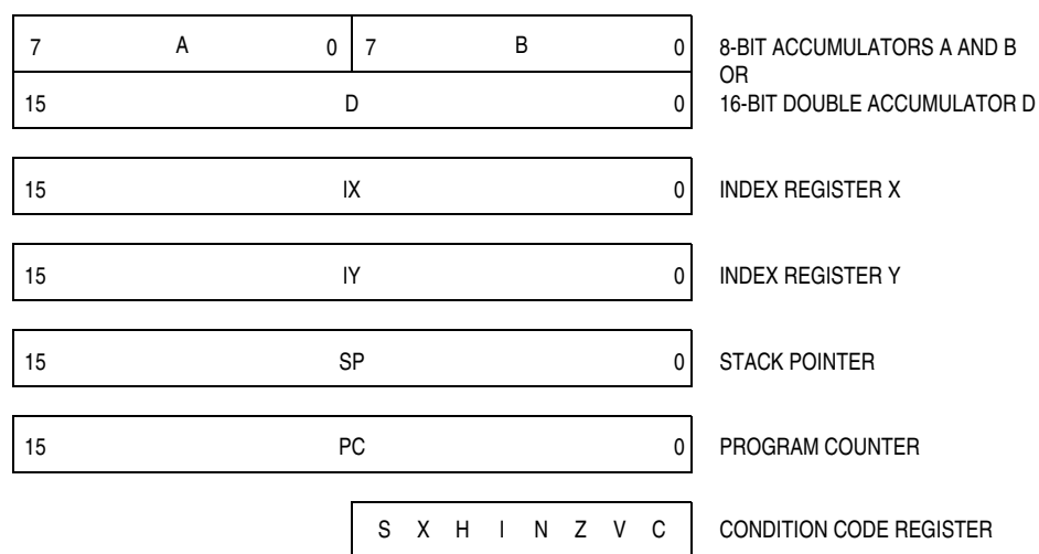
Figure 2-1. Programming Model
