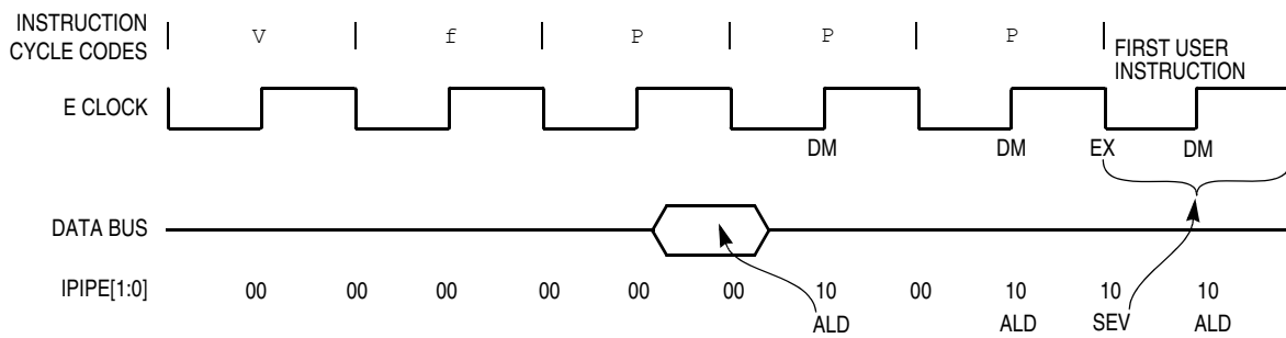
Figure 8-4. Reset Sequence for M68HC12
