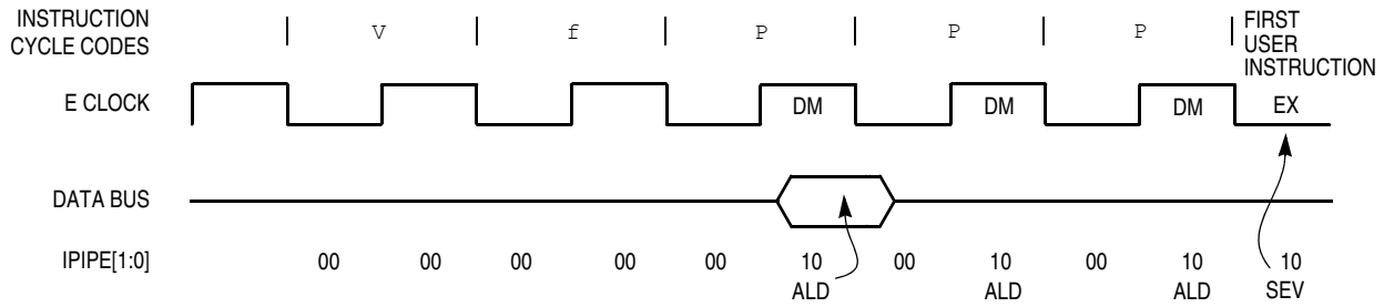
Figure 8-3. Reset Sequence for HCS12
